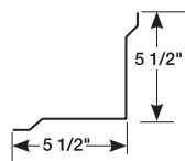
INSIDE CORNER
