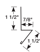
EAVE TRIM
