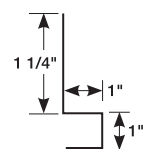
STARTER STRIP
