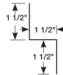
BASE MOULDING
