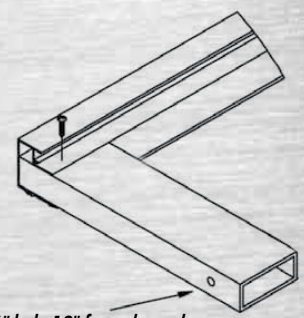
Drill 9/16" hole 12" from the end of the header for trolley hanger (24" for panels wider than 10')
