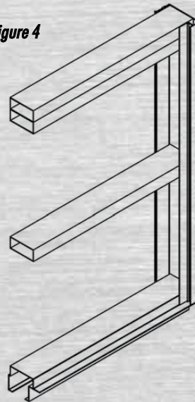
3300 series rail w/ 3394 bottom rail shown with steel box girt
