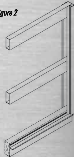
2200 series rail w/ 2201 bottom rail shown with steel box girt
