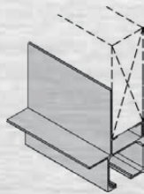
1600WB bottom rail
