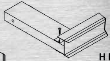
Drill 9/16" hole 12" from the end of the header for trolley hanger (24" for panels wider than 10')
